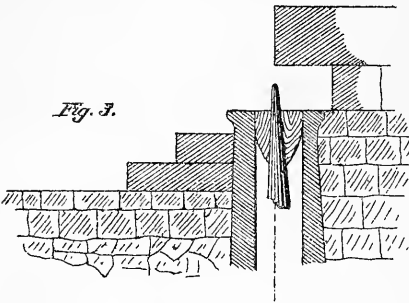
Sketches in place and section of Egyptian pivot-anchors.
